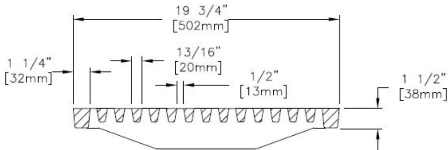
GRATE SECTION
