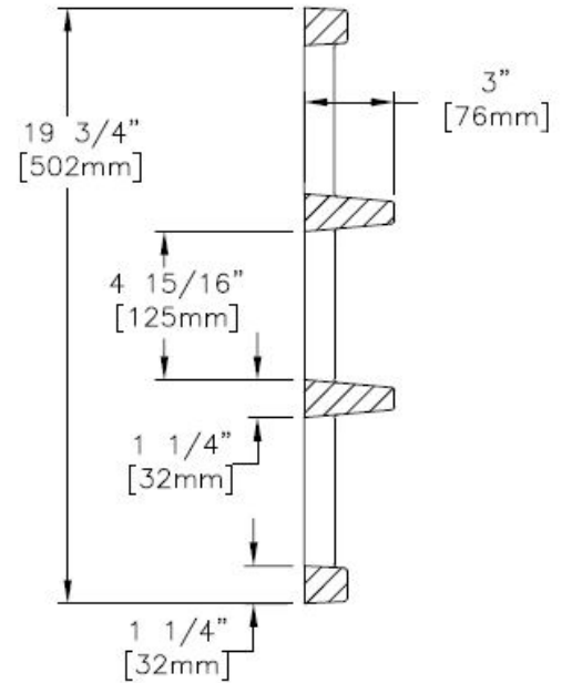
GRATE SECTION
